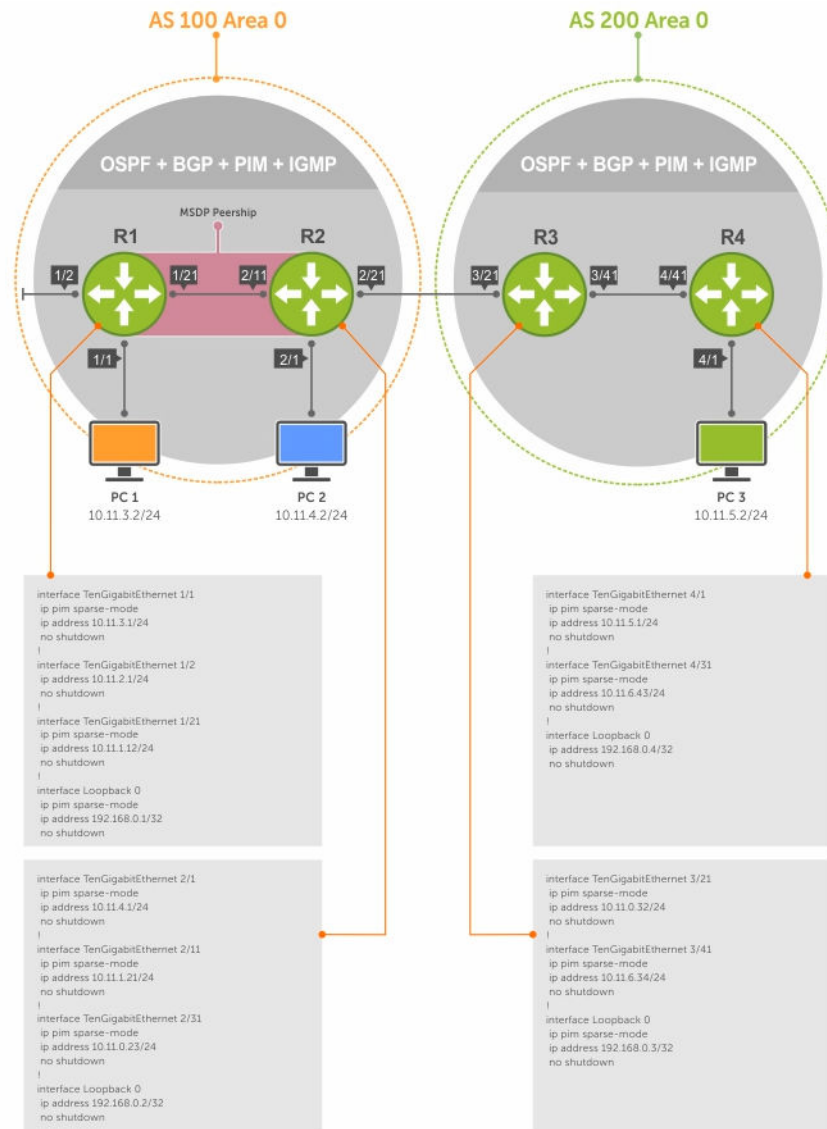
Figure 79. Configuring MSDP
